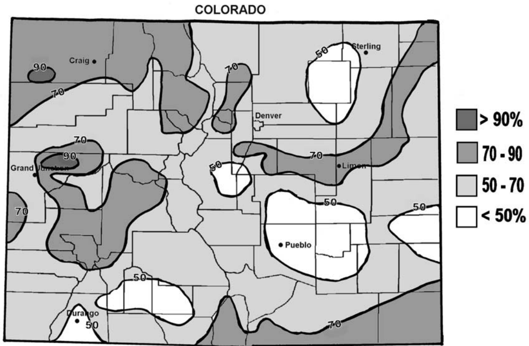
Water Year 2002 (Oct 2001 - Sep 2002) precipitation as a percent of the 1961-1990 averages.
