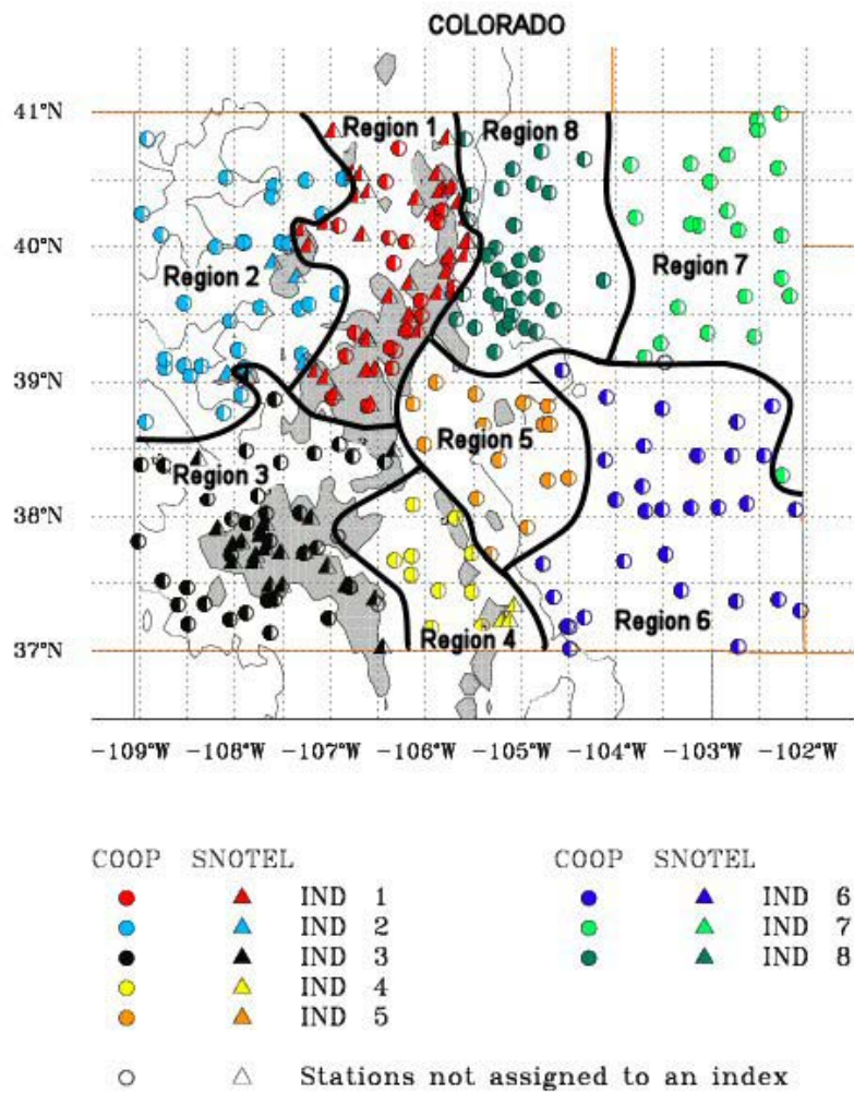
Figure 9. Climate divisions for the state of Colorado (from Klaus Wolter, NOAA-CIRES Climate Diagnostics Center).
