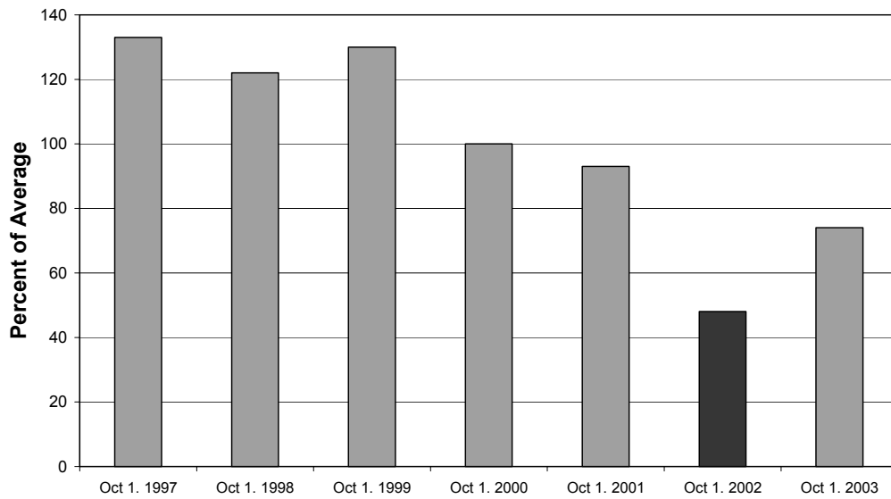
Figure 17. Colorado statewide reservoir storage levels as a percent of average for the end of the growing season (from data provided by the NRCS).
