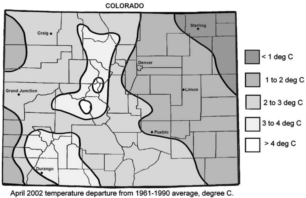
Figure 4. April 2002 temperature departures from the 1961-1990 average for the state of Colorado, USA (degrees C).
