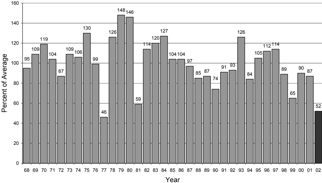
Figure 3. April 1 Snowpack percent of average for state of Colorado for years 1968 through 2002 (from NRCS, Snow Survey Division).
