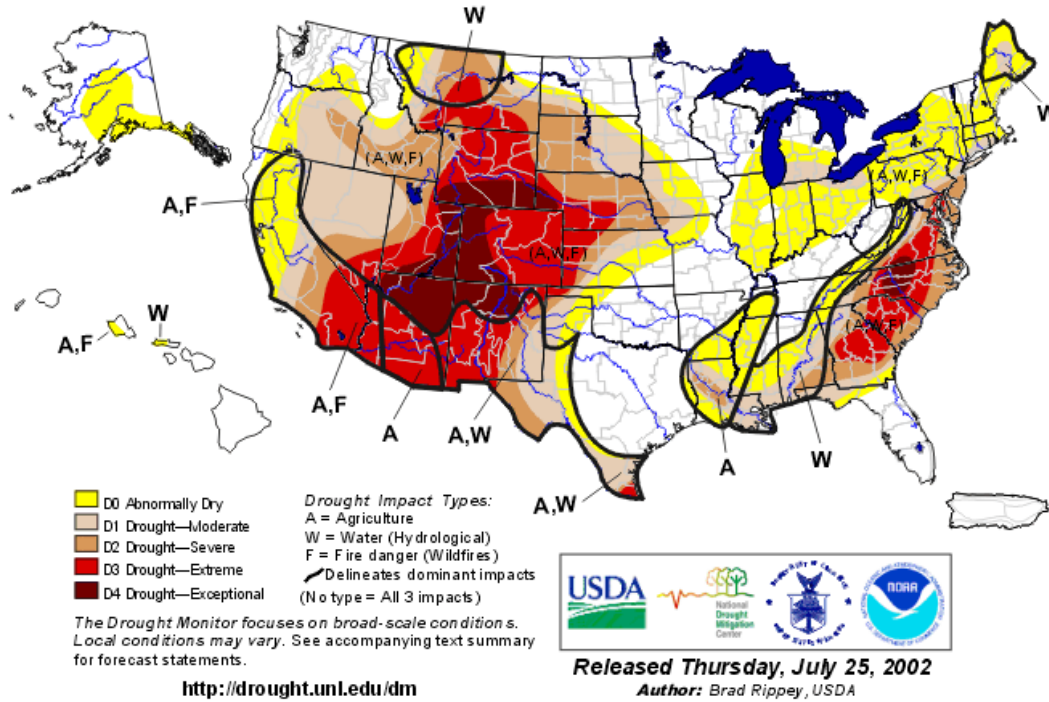
Figure 1. U.S. Drought Monitor for July 23, 2002 shows much of the state of Colorado in “exceptional” D4 drought (from National Drought Monitor, University of Nebraska – Lincoln, http://drought.unl.edu/dm ).
