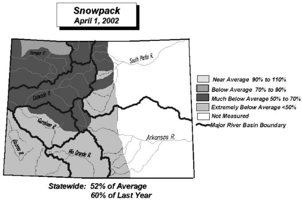
Figure 2. April 1, 2002 snowpack for state of Colorado (from the USDA, National Resources Conservation Service, NRCS, http://www.co.nrcs.usda.gov/snow/data/snmap402.html ).
