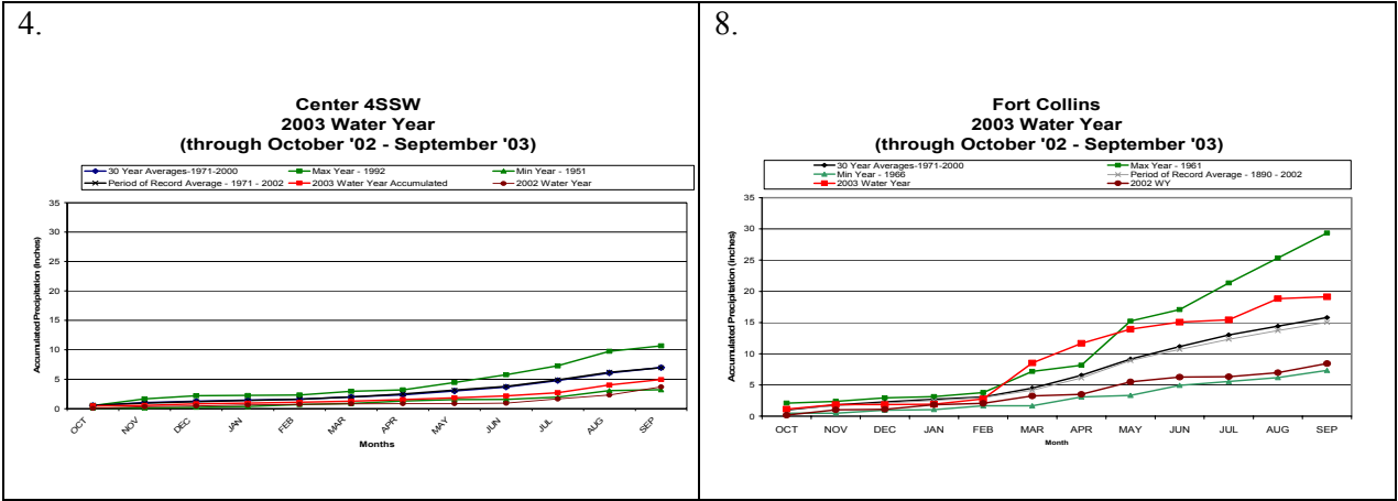
Figure 10. Cumulative precipitation totals for 2002 Water Year, 2003 Water Year 2003, 30-year average, and maximum and minimum years for regions (1) Grand Lake, (2) Meeker, (3) Mesa Verde National Park, (4) Center, (5) Pueblo, (6) Rocky Ford, (7) Akron and (8) Fort Collins, Colorado, USA.
