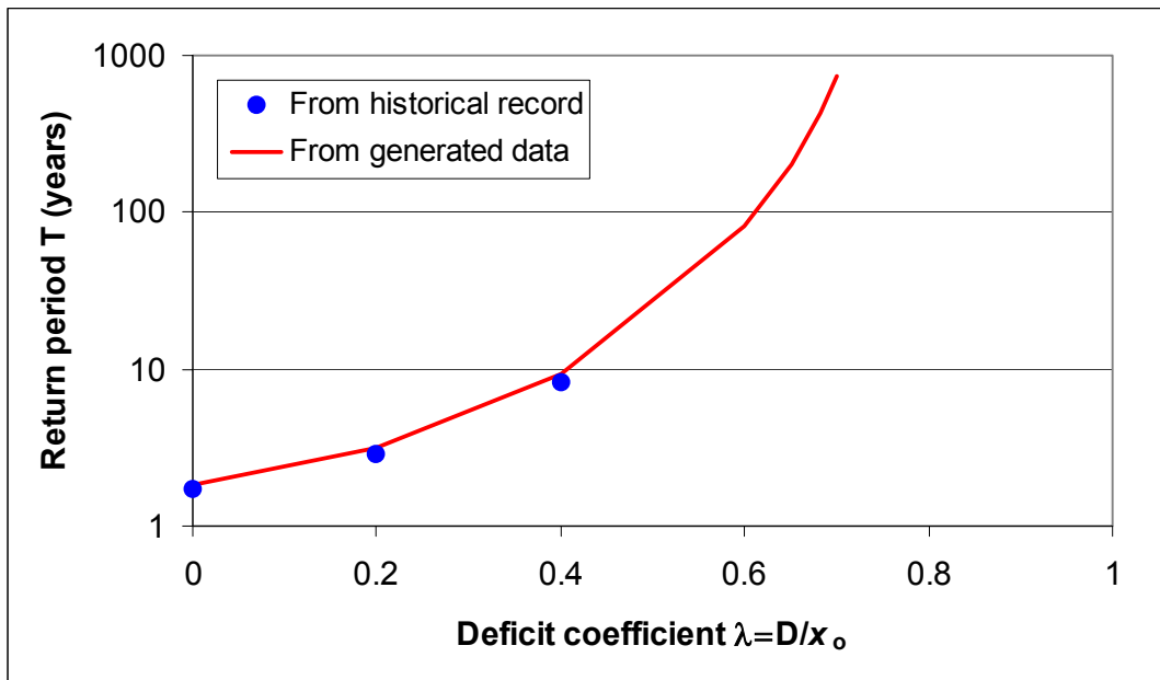
Figure 16. Comparison of the return period ( T ) of single year deficit obtained from the generated flow record versus the T obtained from the historical record for various values of the deficit coefficient \lambda .
