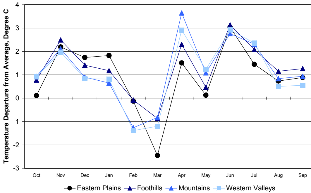
Figure 13. Temperature departures from average for the 2002 Water Year for the Eastern Plains, Foothills, Mountains and Western Valleys. Notice the warm temperatures for April 2002 in the Mountains region, greater than 3°C above average.
