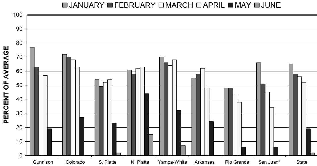
Figure 11. Colorado snowpack summary by basin for January through June 2002 (from USDA, NRCS).
