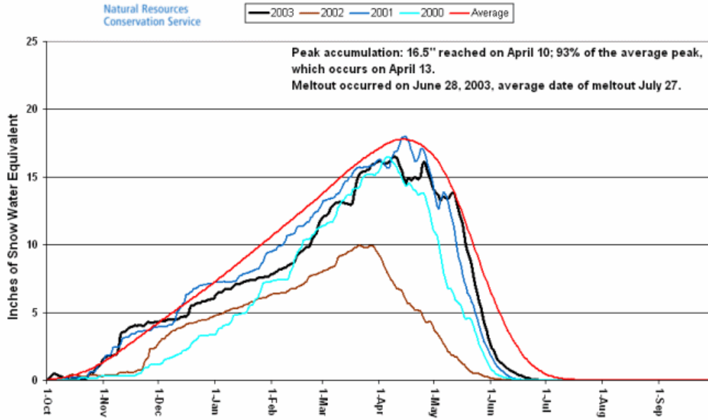
Figure 12. Cumulative statewide snowpack for Colorado for years 1999-2000, 2000-2001, 2001-2002, 2002-2003, and average (from USDA, NRCS).
