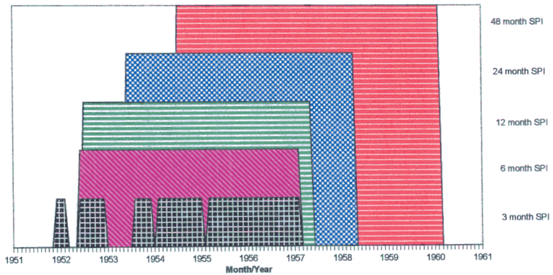
Fig 4.11 (B) 1950s drought at different time scales for McPherson, Kansas.
