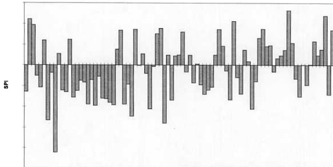
Time Series average 3 month SPI (Aug) all NORTHWEST stations the POR 1911-1995
