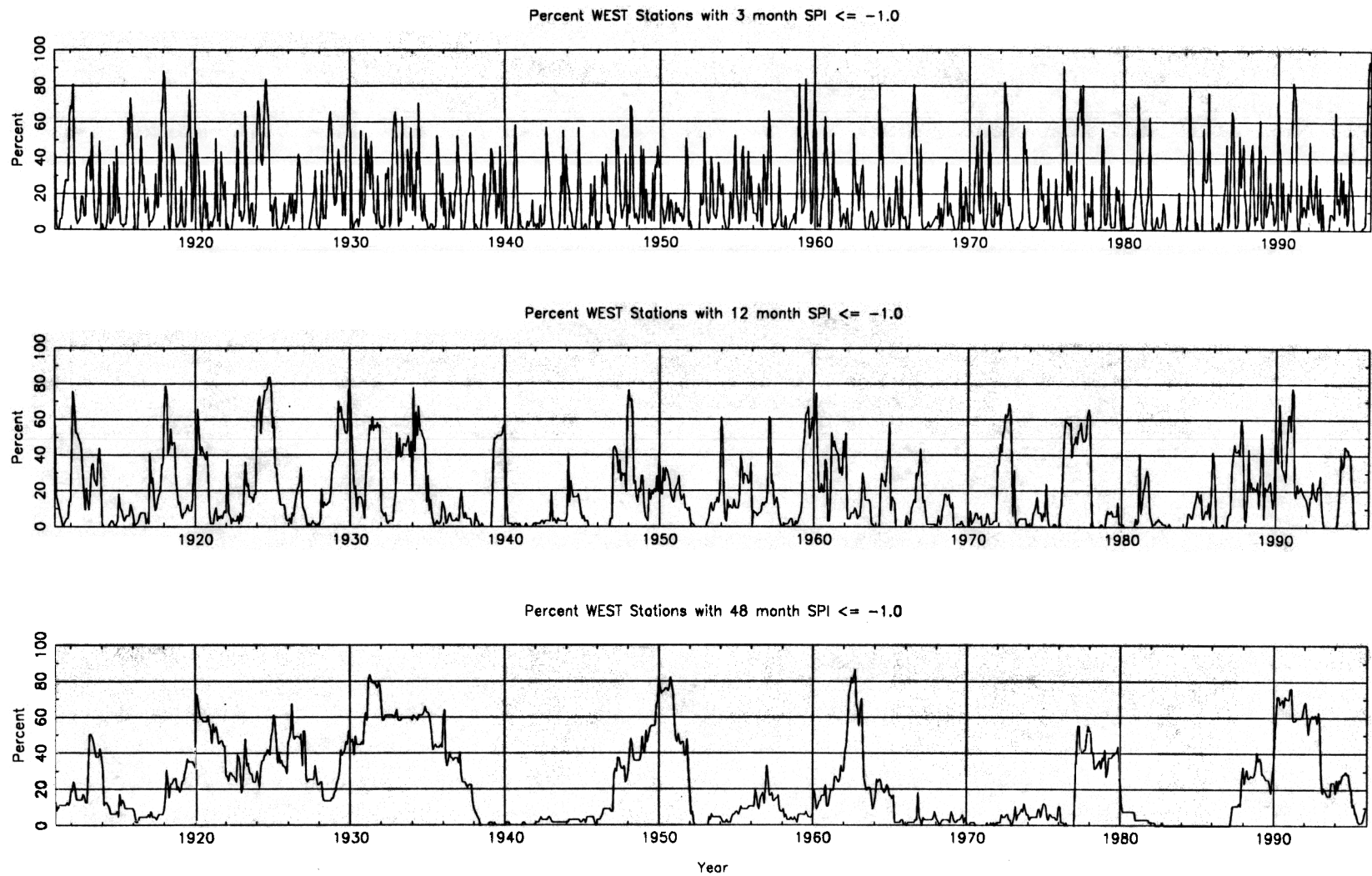
Fig 4.19(A) Time series of percent of all West stations with SPI \leq -1.0 by time scale for the period January, 1911 through December, 1995.
