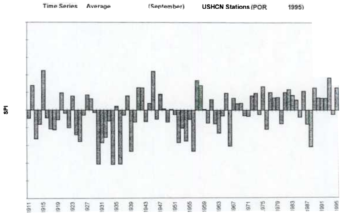
Fig (A) Time series of average 6 month SPI for September (spring and summer) of all USHCN stations for the period January, 1911 through December, 1995
