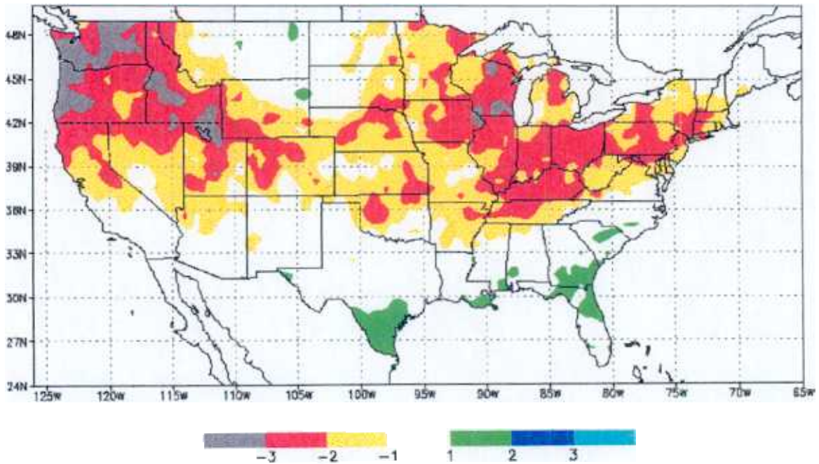
3 Month SPI: JAN 1977
