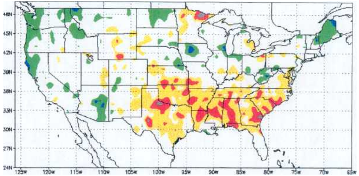
3 Month SPI: AUG 1954
