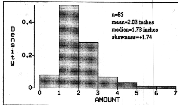
Frequency distribution of 3 month precipitation amounts (inches) for the month of March (totals for January, February, and March) for Fort Collins, CO for the years 1911 through 1995.
