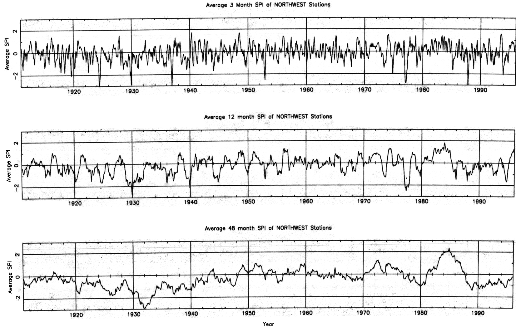
Fig 4.21(B) Time series of average SPI of all Northwest stations by time scale for the period January, 1911 through December, 1995.
