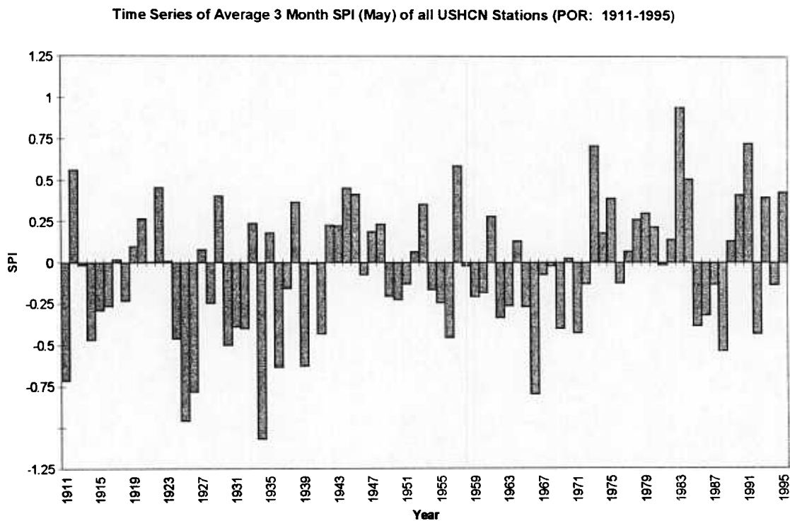
Fig 4.15 (B) Time series of average 3 month SPI for May (spring) of all USHCN stations for the period January, 1911 through December, 1995.
