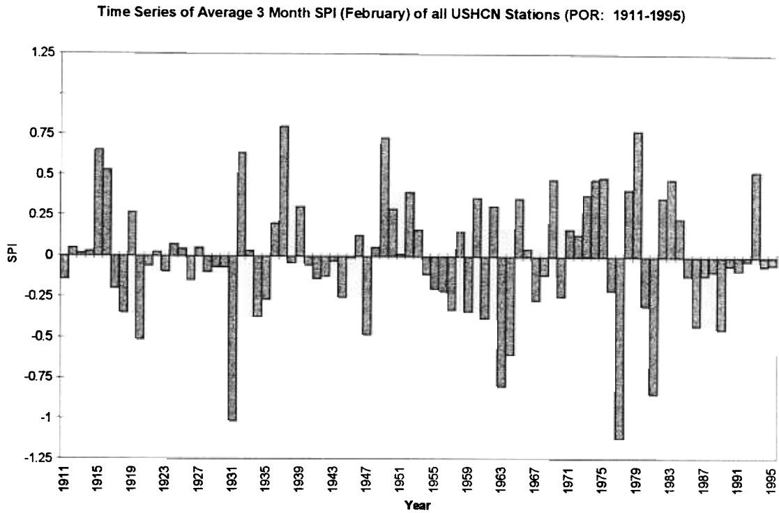
Fig 4.15 (A) Time series of average 3 month SPI for February (winter) of all USHCN stations for the period January, 1911 through December, 1995.
