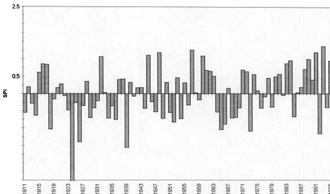
Fig 24(B) Time series of average month SPI for May (spring) of all Northwest stations for the period January, 1911 through December, 1995
