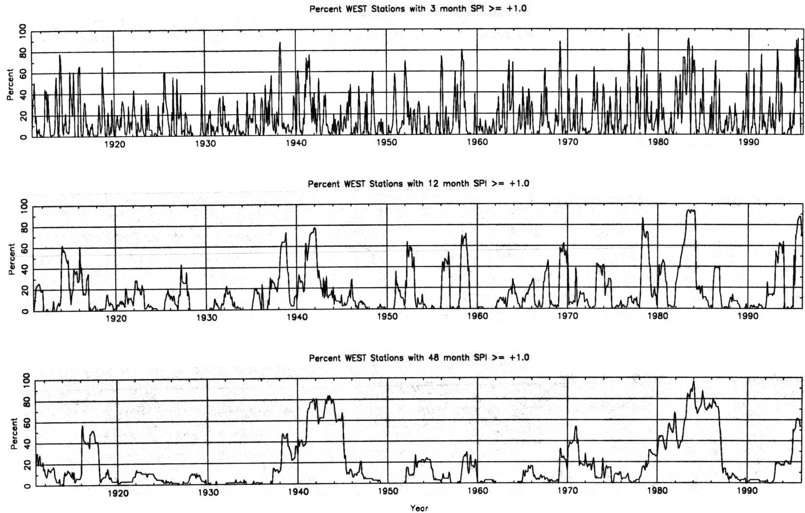
Fig 4.20(A) Time series of percent of all West stations with SPI \geq +1.0 by time scale for the period January, 1911 through December, 1995.
