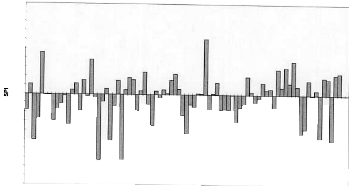
Time Series average 3 month SPI (August) CENTRAL stations the POR 1911-1995
