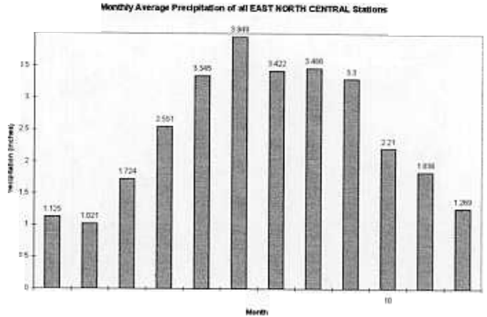
Fig 4.17(G) Annual distribution of monthly average precipitation of all East North Central stations for the period January, 1911 through December, 1995.
