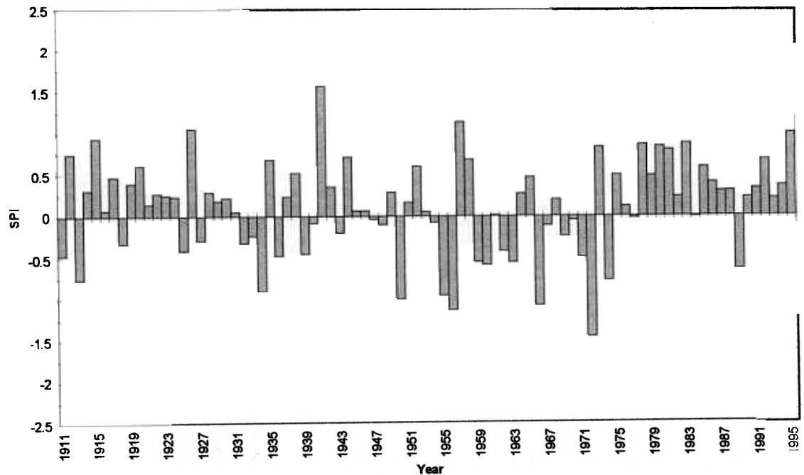
Fig 4.26(B) Time series of average 3 month SPI for May (spring) of all Southwest stations for the period January, 1911 through December, 1995.
