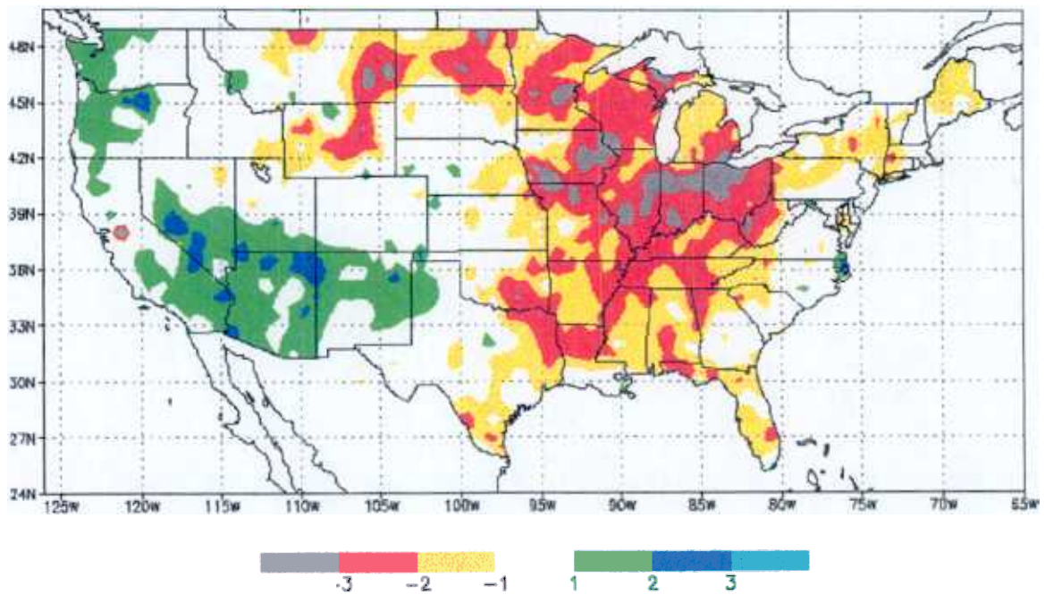
3 Month SPI: JUN 1988
