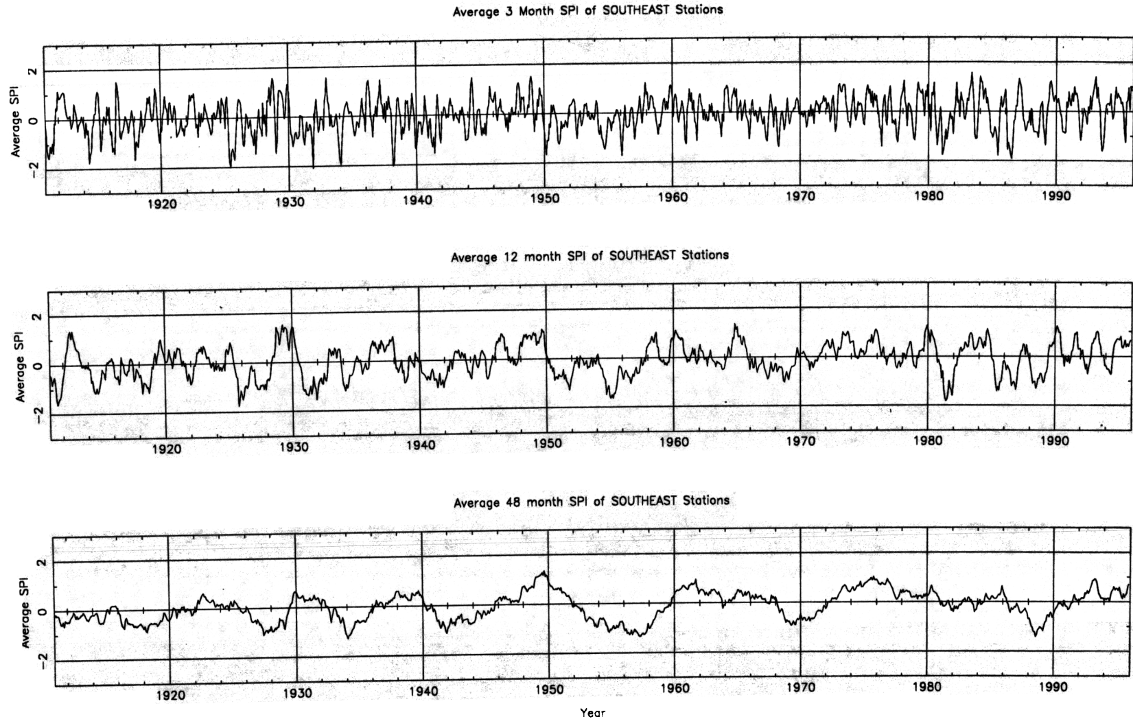
Fig 4.21(I) Time series of average SPI of all Southeast stations by time scale for the period January, 1911 through December, 1995.
