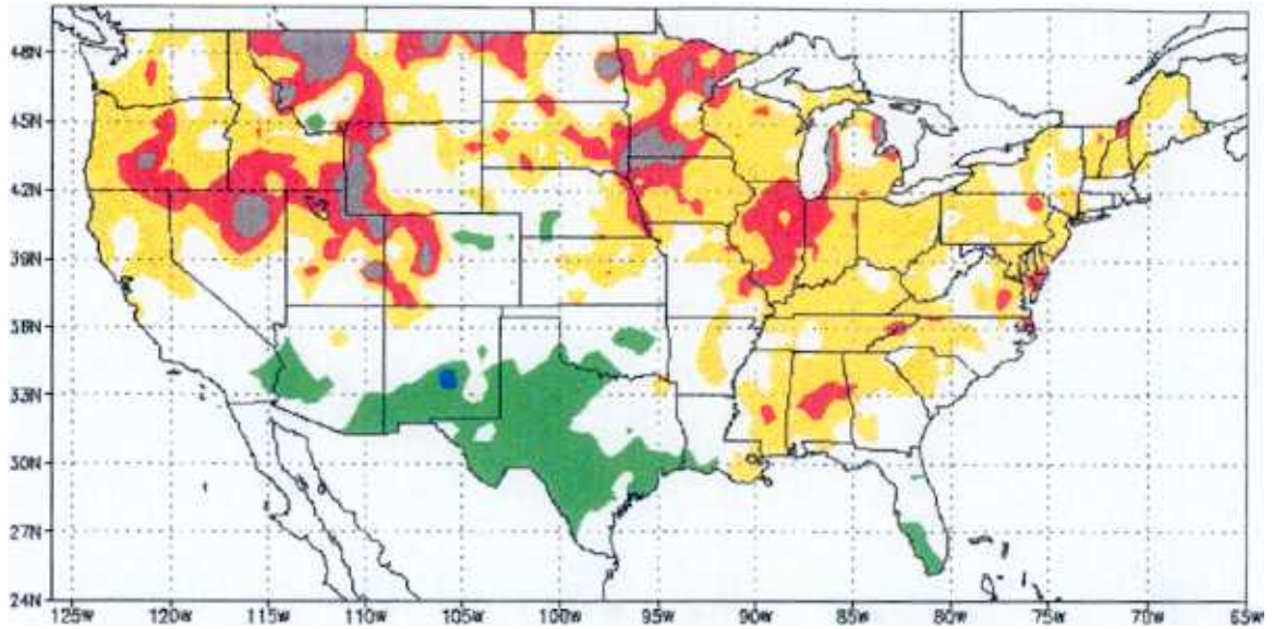
3 Month SPI: FEB 1931
