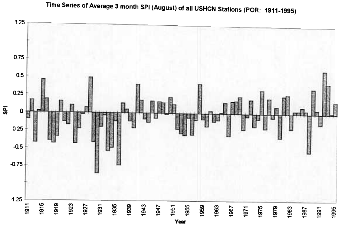
Fig 4.15 (C) Time series of average 3 month SPI for August (summer) of all USHCN stations for the period January, 1911 through December, 1995.
