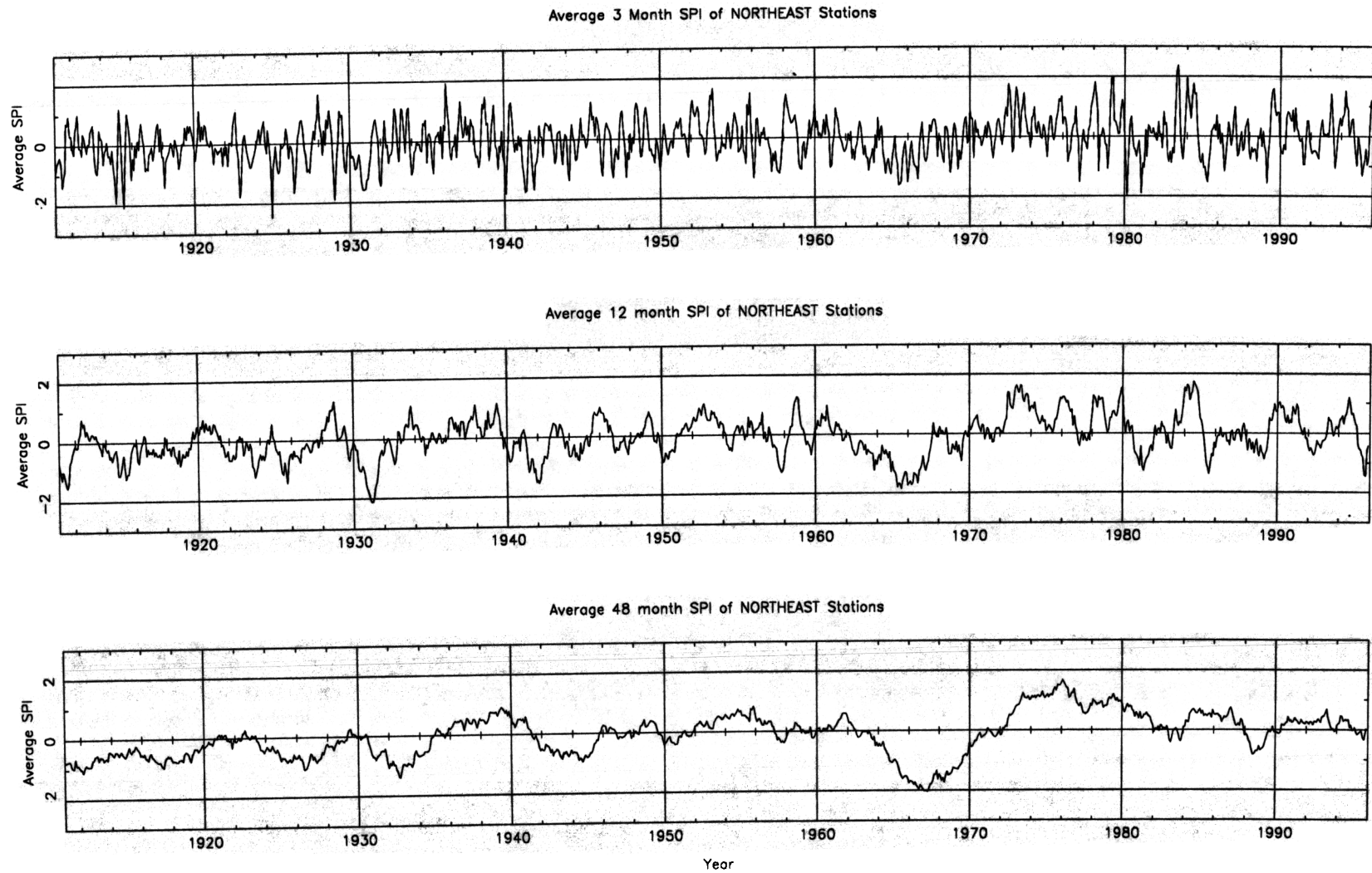
Fig 4.21(H) Time series of average SPI of all Northeast stations by time scale for the period January, 1911 through December, 1995.
