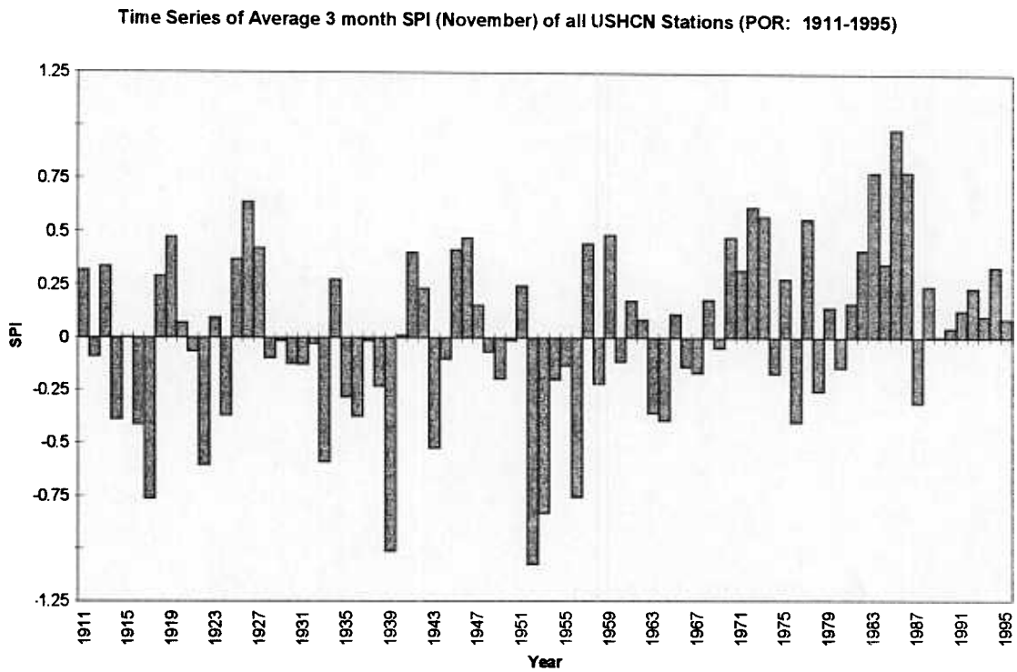
Fig 4.15 (D) Time series of average 3 month SPI for November (autumn) of all USHCN stations for the period January, 1911 through December, 1995.
