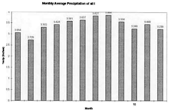
Fig 4.17(H) Annual distribution of monthly average precipitation of all Northeast stations for the period January, 1911 through December, 1995.
