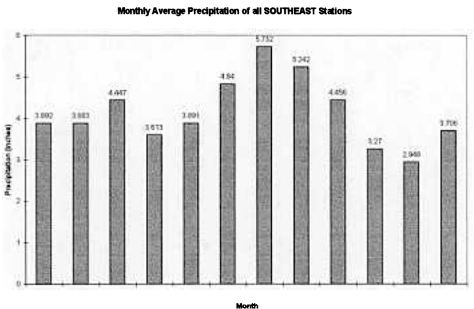
Fig 4.17(I) Annual distribution of monthly average precipitation of all Southeast stations for the period January, 1911 through December, 1995.
