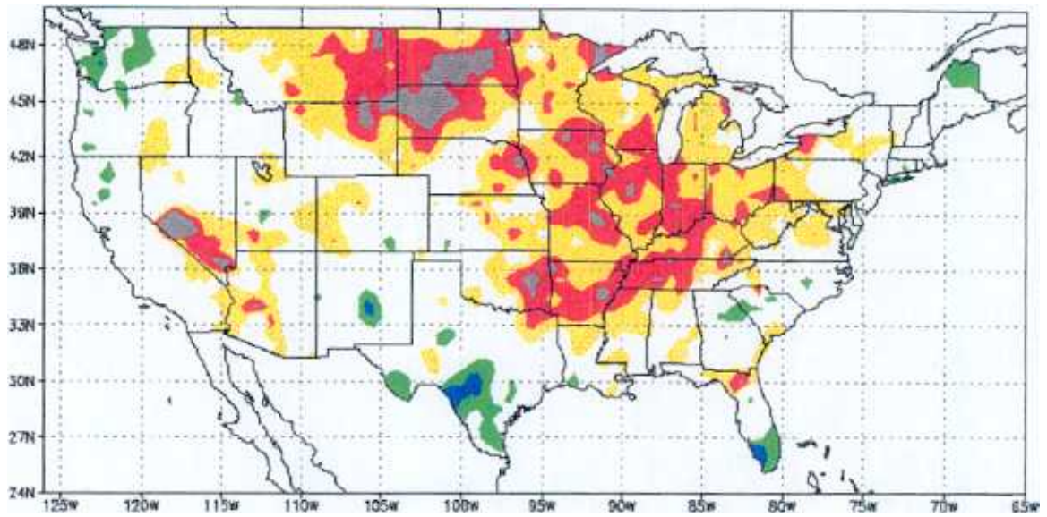
3 Month SPI: JUN 1936
