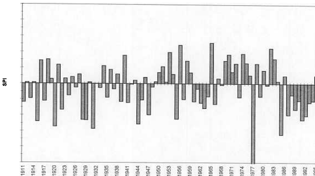
Fig 4.24(A) Time series of average month SPI for February (winter) of all Northwest stations for the period January, 1911 through December, 1995
