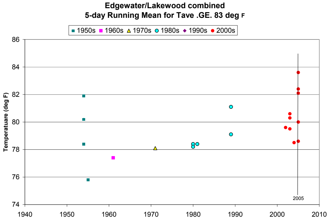
Figure 7. Time series of 5-day centered mean daily temperatures ( ^{\circ}\text{F} ) for each day with a mean temperature (average of the high and low for the day) of 83^{\circ}\text{F} or higher. This time series incorporates data from the Edgewater, CO, cooperative weather station 1948-1962 and the nearby Lakewood, CO, cooperative station from 1962-2005.
