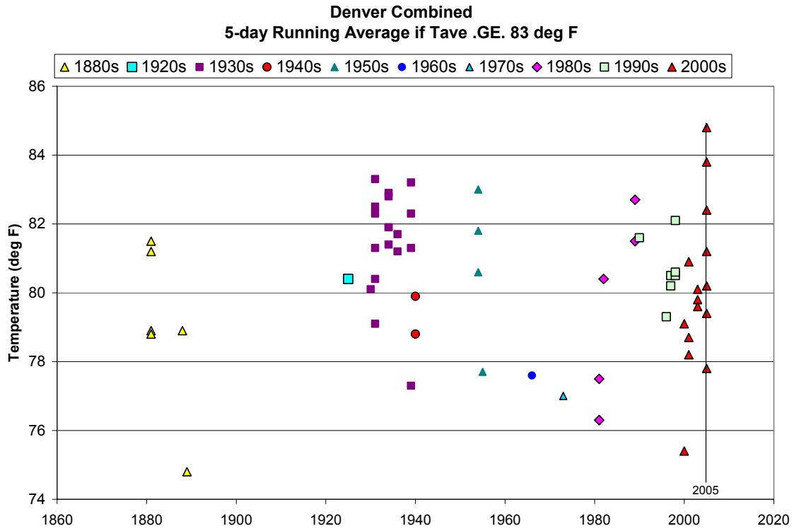
Figure 6. Time series, 1872-2005, of 5-day centered mean daily temperatures ( ^{\circ}\text{F} ) for each day with a mean temperature (average of the high and low for the day) of 83^{\circ}\text{F} or higher. This time series incorporates data from the original downtown Denver weather station from 1872-1950 with Denver Stapleton data (1950-1995) and Denver International airport (1995-2005).
