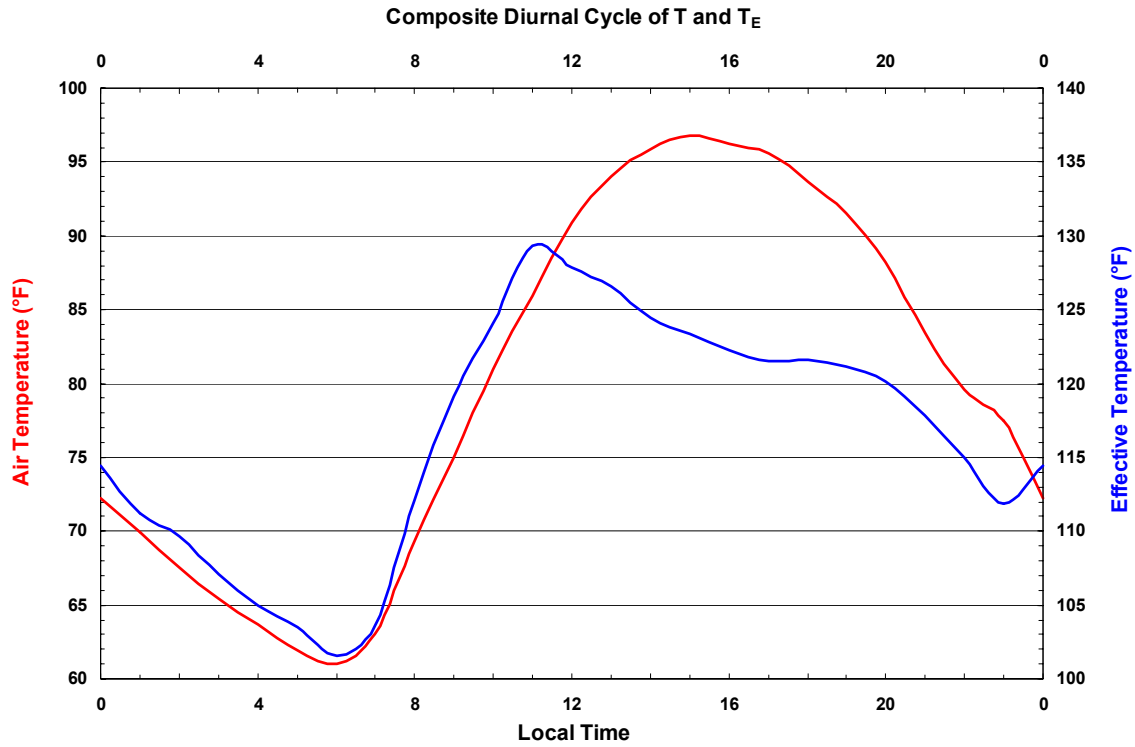
Figure 10. A daily composite of air temperature (red line) and effective temperature (blue line). The composite is created by averaging hourly data during the five days with highest air temperature in each of the three years considered in this section – fifteen days total. This shows the pattern of heating and cooling on the station’s extreme hottest days. Note how the effective temperature peaks approximately four hours before the air temperature peaks. Typically, the hottest days are characterized by exceptionally low relative humidity in the late afternoon, which explains the premature drop in effective temperature.
