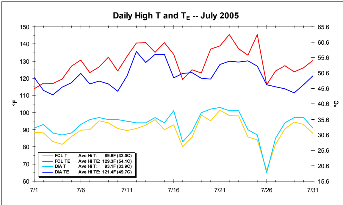
Figure 9. Hourly data from automated weather stations at FCL and DIA are used to pick and calculate the highest air temperature and effective temperature for each day in July 2002 (a), July 2003 (b), and July 2005 (c). In all three months, the average high air temperature is higher at DIA, while the average high effective temperature is higher at FCL.
