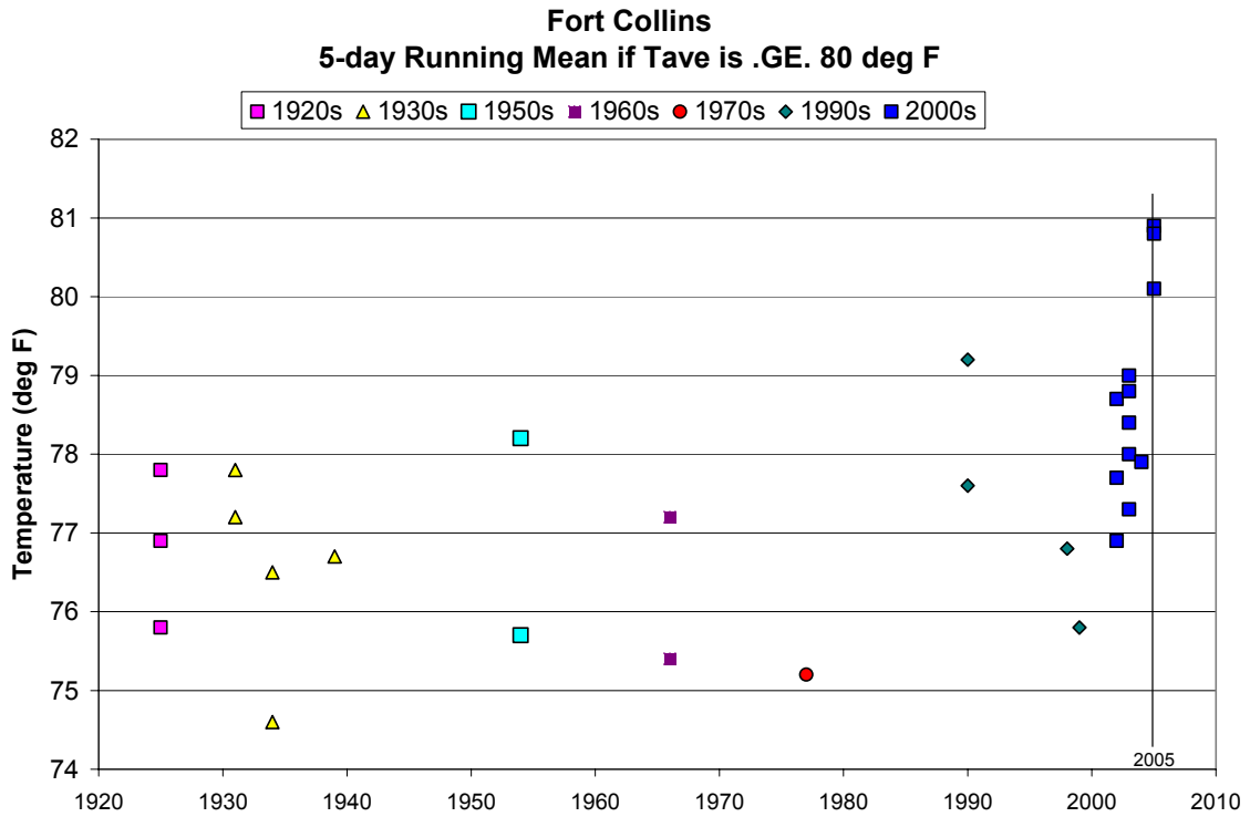
Figure 8. Time series, 1889 – 2005, of 5-day centered mean daily temperatures (°F) for the Fort Collins, CO weather station for each day with a mean temperature (average of the high and low for the day) of 80°F or higher. The threshold of 80°F or higher was used because there were no days above 83°F.
