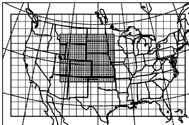
Figure 1. Regional Atmospheric Modeling System (RAMS) simulation domain and grid configuration. Coarse and fine-grid intervals are 200 km and 50 km, respectively.
