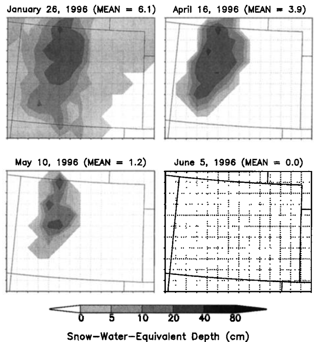
Figure 7. RAMS simulation of the temporal evolution of snow-water-equivalent distribution for the Colorado subdomain for the case where only the January 26, 1996, observed snow-water-equivalent distribution was provided as initial conditions.
