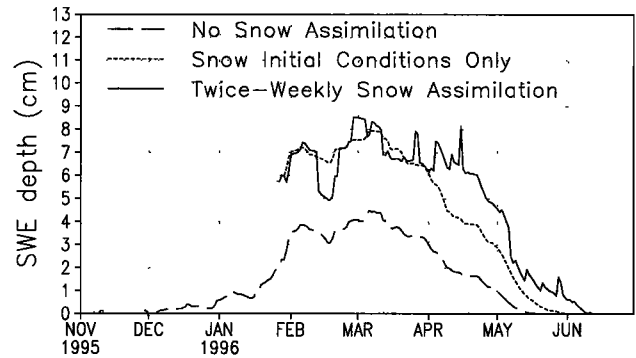
Figure 6. Domain-averaged snow-water-equivalent depth distributions for the Colorado subdomain given in Figure 4 for three RAMS simulations: (1) no assimilation of the observed snow-water-equivalent data (simulation running from September 1, 1995 to June 30, 1996), (2) the snow initial conditions given by the January 26, 1996, observed snow-water-equivalent distribution (simulation running from January 16 to June 30, 1996), and (3) observed snow-water-equivalent distributions assimilated when available, as defined in Figure 3 (simulation running from January 16 to June 30, 1996).
