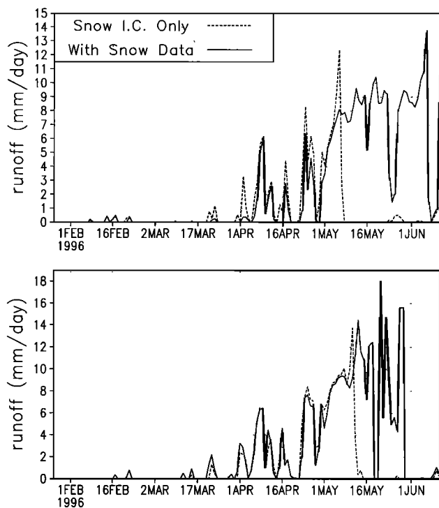
Figure 12. Temporal evolution of runoff for the RAMS grid cells represented by (top) the circle and (bottom) the square markers in Figures 5 and 12 for the two simulations identified in Figure 8.
