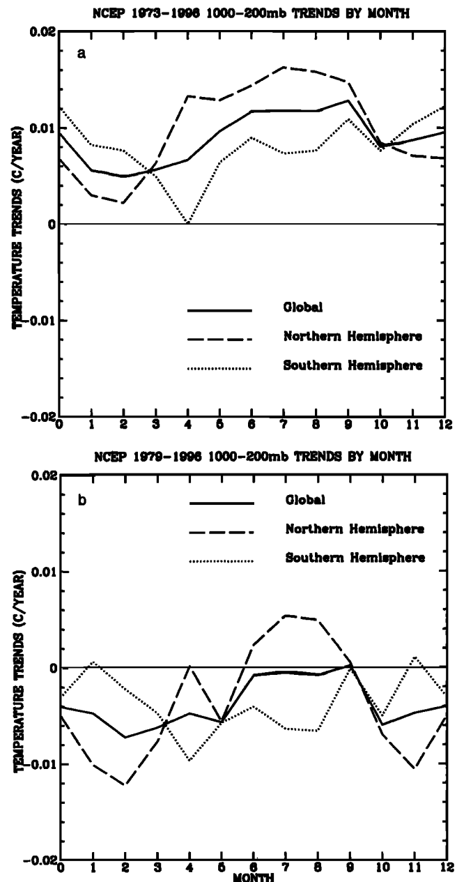
Figure 2. Global and northern and southern hemispheres monthly 1000–200 mbar layer temperature trends ( ^{\circ}\text{C yr}^{-1} ) calculated from the NCEP reanalysis for (a) 1973–1996, and (b) 1979–1996. Months are plotted along the x axis (0 = December, 1 = January, ..., 12 = December).
