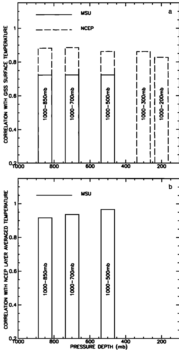
Figure 4. (a) Pearson's correlation coefficients for NCEP and MSU between 1000 mbar and the indicated level with the surface record. (b) Pearson's correlation coefficients between NCEP and lower-troposphere MSU data between 1000 mbar and the level indicated; MSU comparison with the two deeper layers have been omitted. (The MSU data correspond to only one averaged lower-tropospheric layer; see Christy et al. [1998, Figure 1] for the weighting function.)
