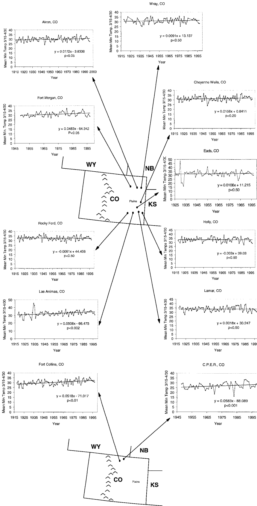
FIG. 1. Spring mean minimum temperatures (°F) for 15 Mar–30 Apr for eastern Colorado locations.
