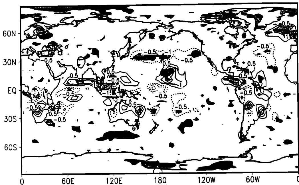
Figure 16. Convective precipitation differences (current minus natural, contour by 0.5 mm d -1 ) using a nine-point spatial filter for easier visibility. Lighter shading represents the 90% significance level for a one-sided t -test. Darker shading represents the 95% significance level. Reprinted from Chase et al. [2000] with permission from Springer-Verlag.
