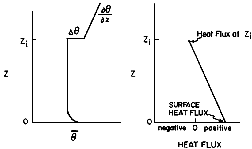
Figure 3. The potential temperature and heat flux profiles assumed in the “jump” model. Reprinted from Pielke [1984] with permission from Academic Press.
