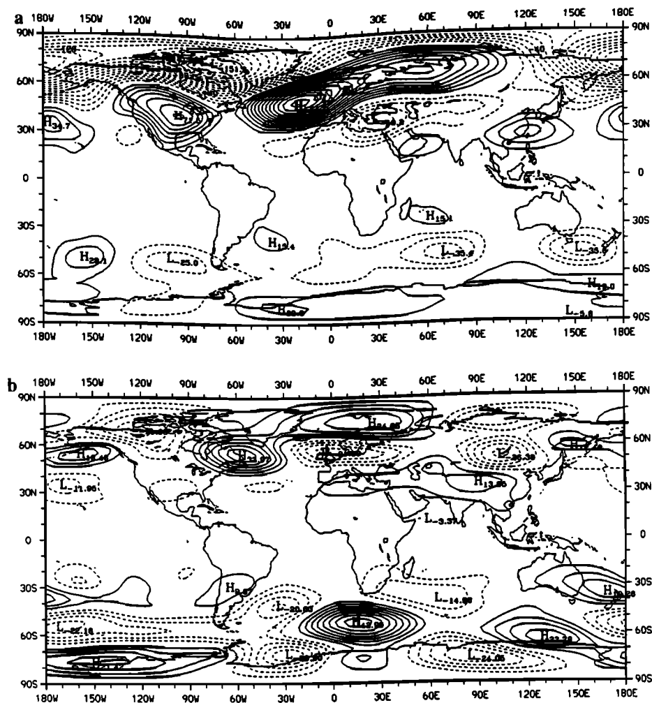
Figure 14. Ten-year averaged differences in 500-mbar height zonal wave numbers 1–6 only (actual LAI minus potential LAI). (a) January, contour 10 m. (b) July, contour 5 m. From Chase et al. [1996].
