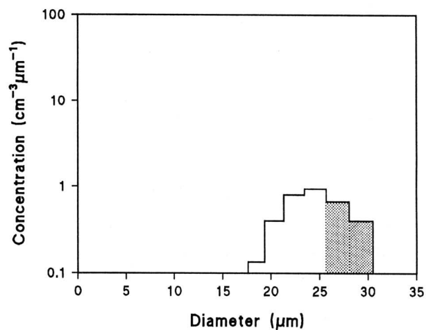
FIG. 10. The photographs and graphs illustrate the effect the size distribution of supercooled water droplets has on the accretion of ice on aircraft. The starboard propeller spinner of the University of Wyoming King Air is shown for two days during WISP, 13 February (upper right panel) and 27 February (upper left panel) 1990, along with representative droplet size distributions measured from a Forward Scattering Spectrometer Probe. The icing for the 13 February case extends farther back on the prop spinner's surface than for 27 February; this represents a more serious icing condition. For 27 February, the aircraft spent 32 min in cloud with an average liquid water content (measured from a King liquid water probe) of 0.29 \text{ g m}^{-3} ; on 13 February, the aircraft spent 51 min in cloud with an average 0.14 \text{ g m}^{-3} liquid water content.
