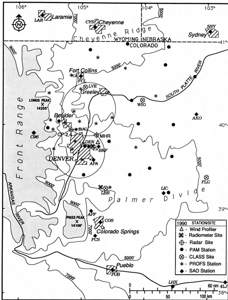
Fig. 1. Winter Icing and Storm Project (WISP90) network of instruments showing the location of the Doppler radars, CLASS stations, PAM and PROFS mesonet stations, radiometer sites, wind profiler sites, and SAO stations. Topographic contours are given every 2000 ft. The shaded region represents terrain above 9000 ft.
