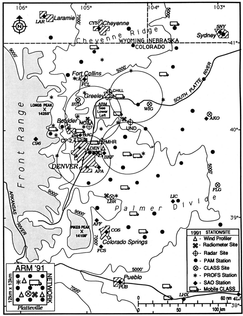
FIG. 2. Same as Fig. 1 except for WISP91.
