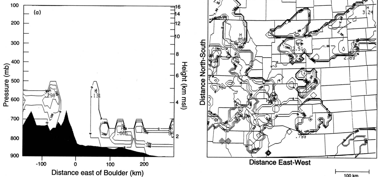
FIG. 5. LAPS model-calculated liquid water content from 6 March 1990: (a) East-west vertical cross section through Boulder at 2300 UTC. Contour interval is 0.1 \text{ g m}^{-3} . (b) Vertically integrated cloud water in mm at 0100 UTC.
