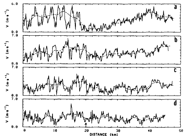
FIG. 15. As in Fig. 12, except for wind speed (the dashed line indicates a subjective estimate of the running mean).
