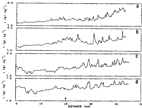
FIG. 8. As in Fig. 7, except for moisture mixing ratio.
