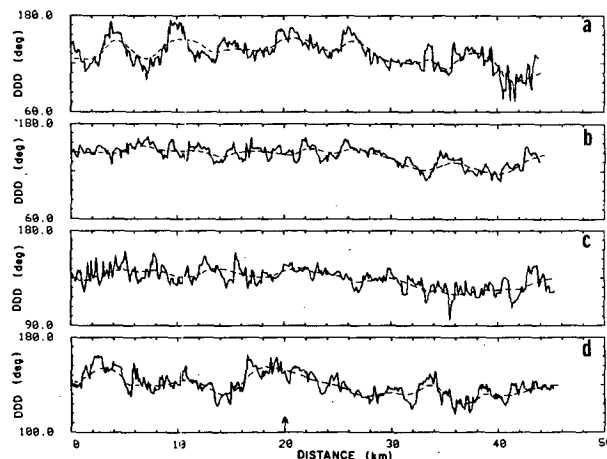
FIG. 9. As in Fig. 7, except for wind direction (the dashed line indicates a subjective estimate of the running mean).
