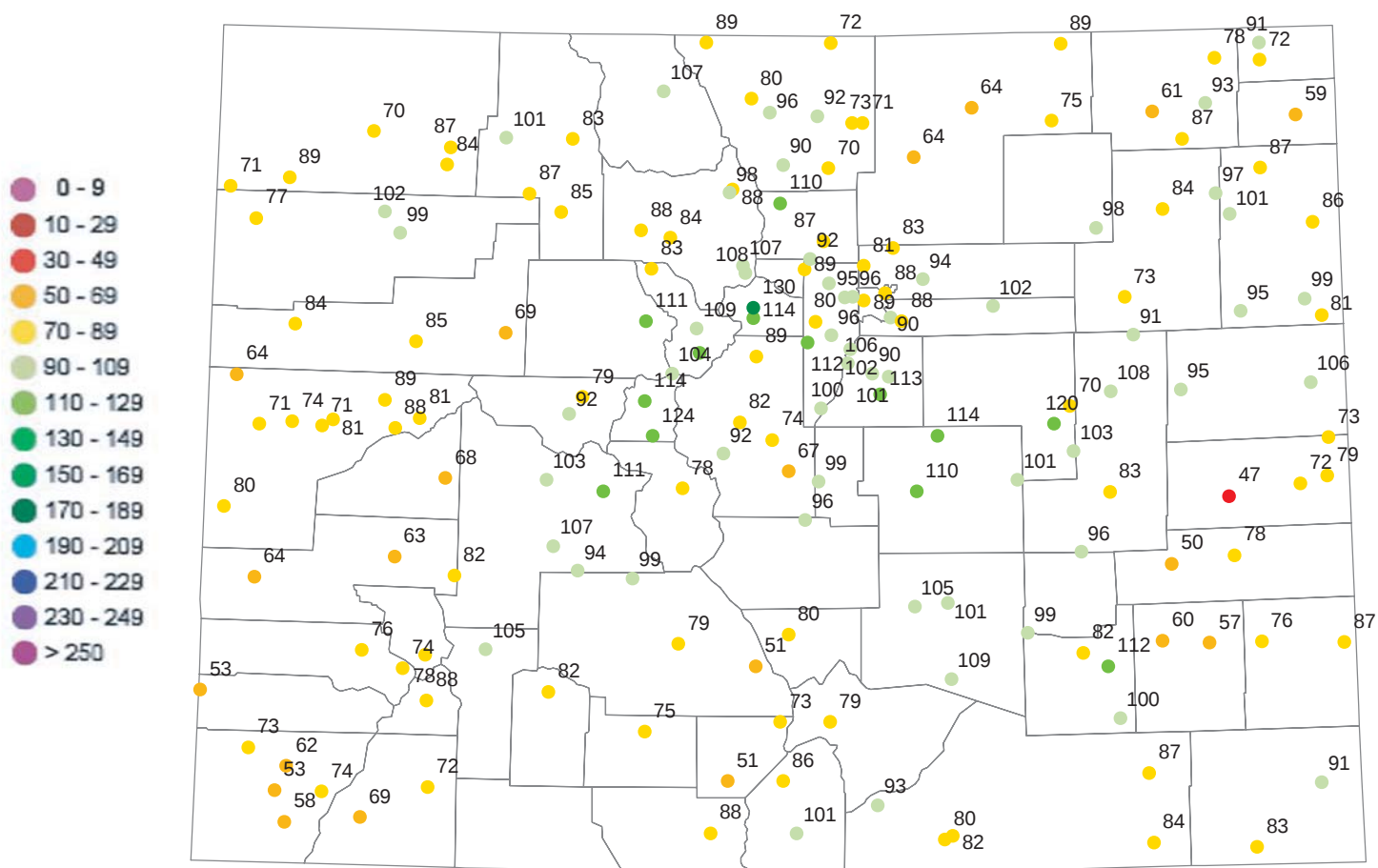
Water Year 2000 (Oct. 1999 - Sept. 2000) precipitation as percent of average for the 1961-1990 averages.
